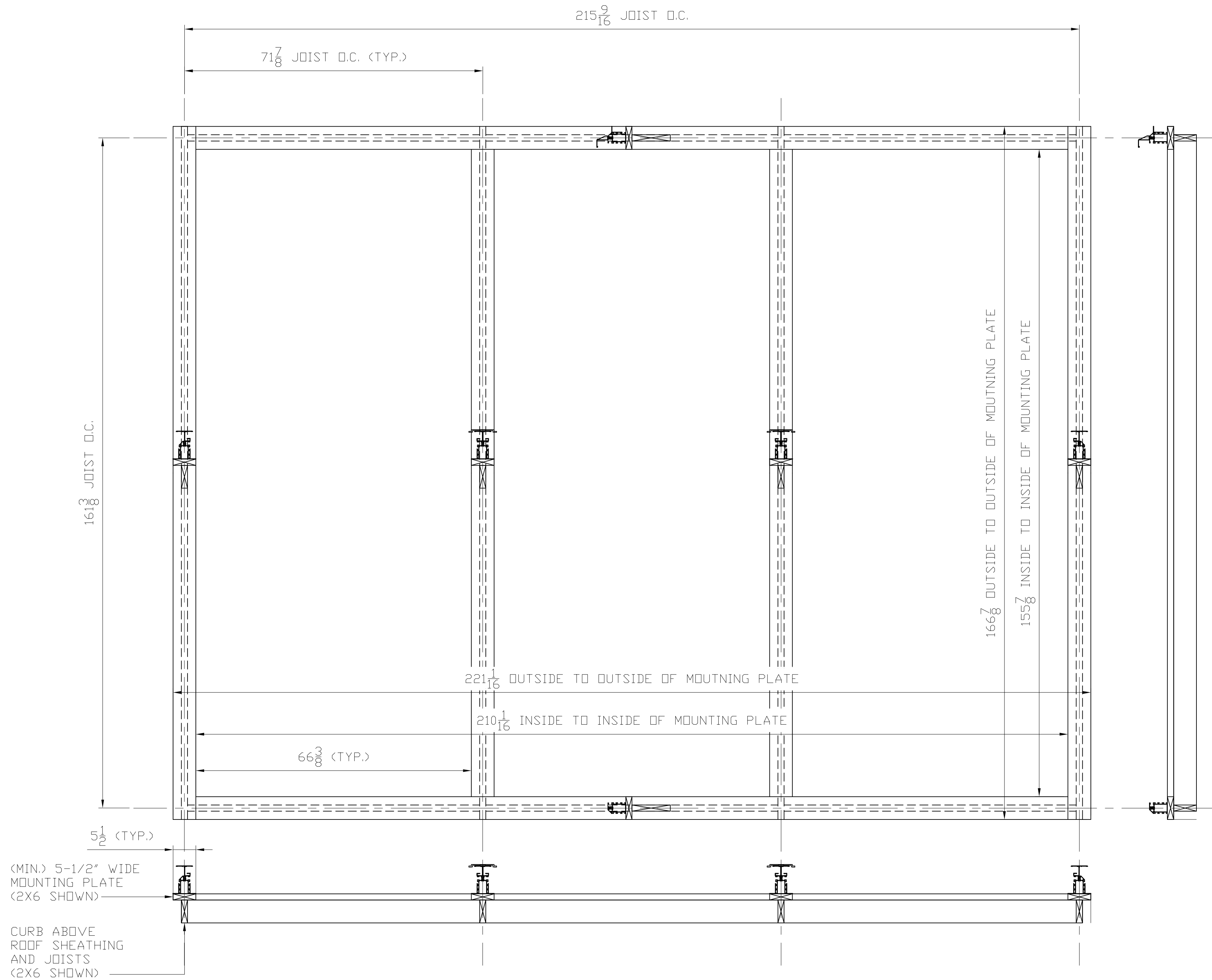
SLIDING ROOF PANEL MOUNTING DETAIL
